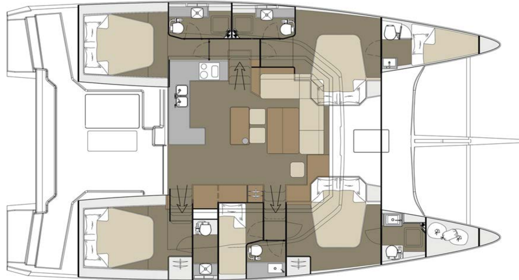
BOAT LAYOUT
